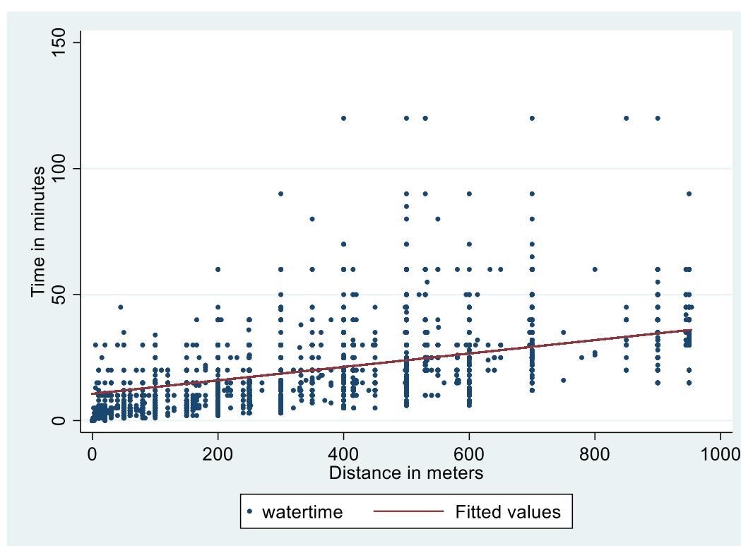
Figure 4. Regression model of time to collect water against distance
